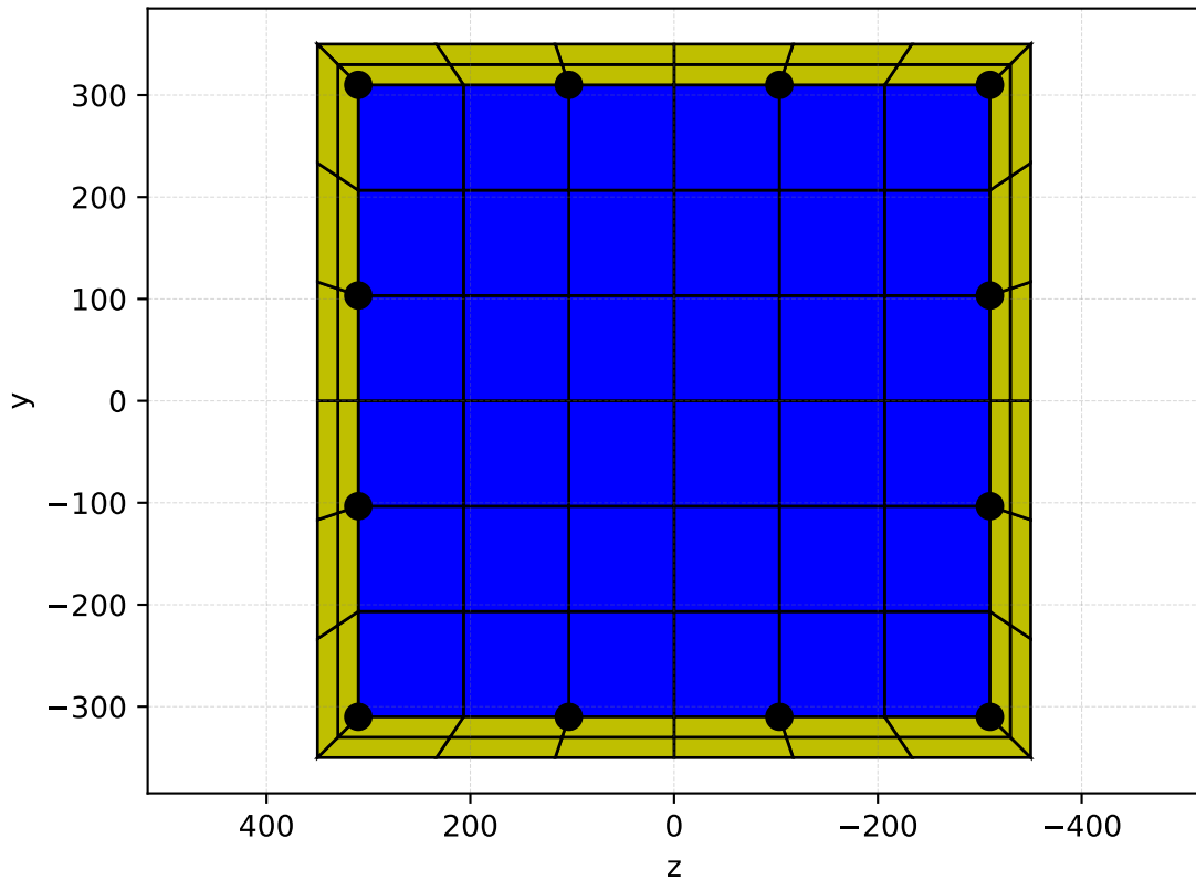
Column Section for Staging
